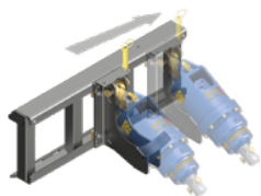
Universal Slide Mount Earth Drill frame to Suit Skidsteer Loader
